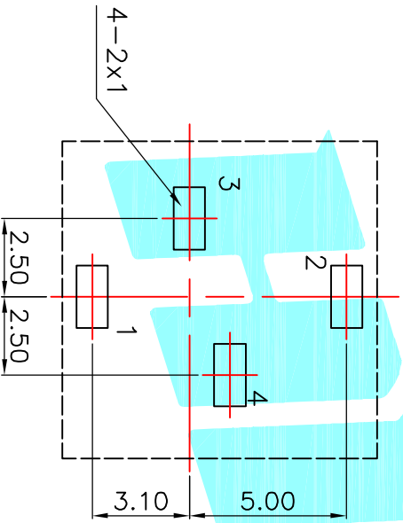
P.C.B LAYOUT(copper-sided view)
